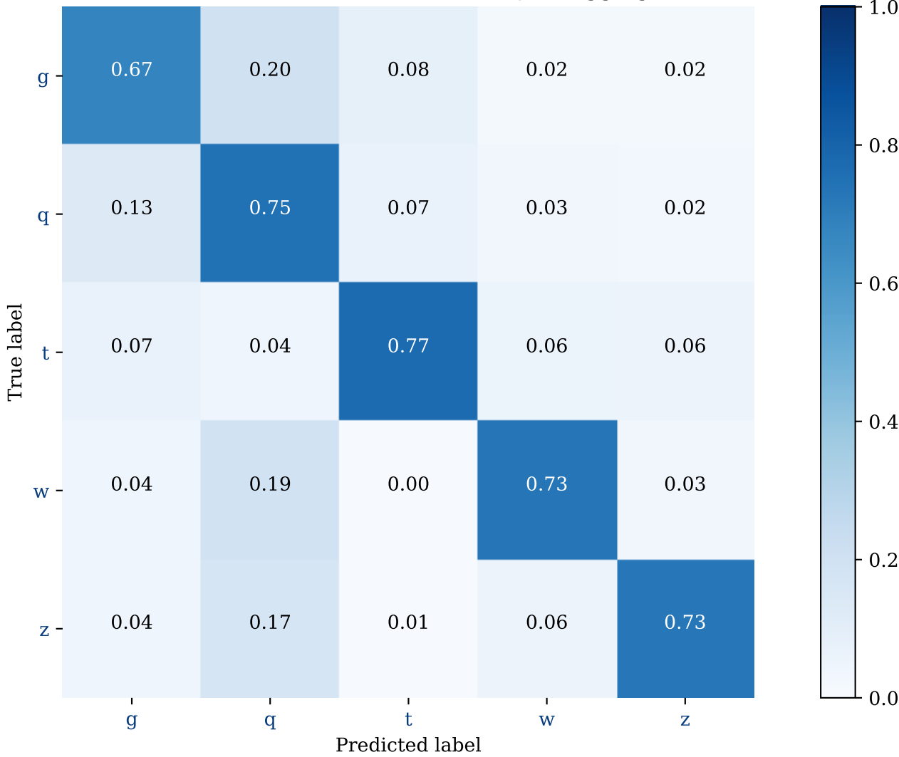
Confusion Matrix of Inference on FPGA with Jet Tagging QKeras-model
